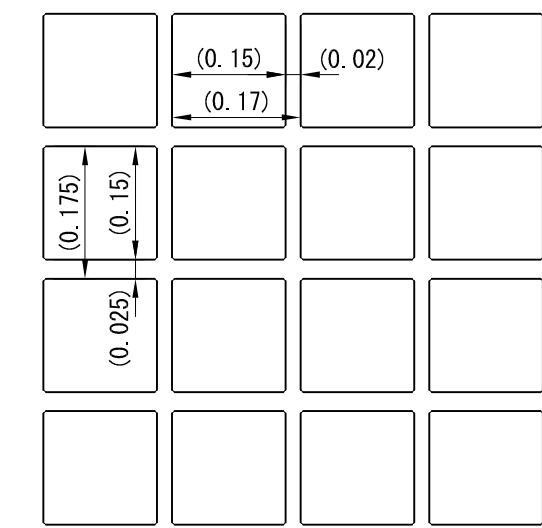
A部拡大図 (100 : 1) A-Portion Magnified Drawing (100:1)
