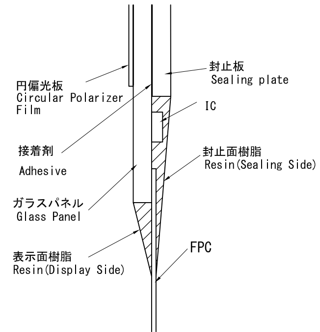
B部拡大図 (10 : 1) B-Portion Magnified Drawing (10:1)
