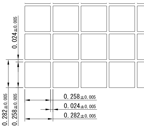
A部拡大図 (50 : 1) A-Portion Magnified Drawing (50:1)
