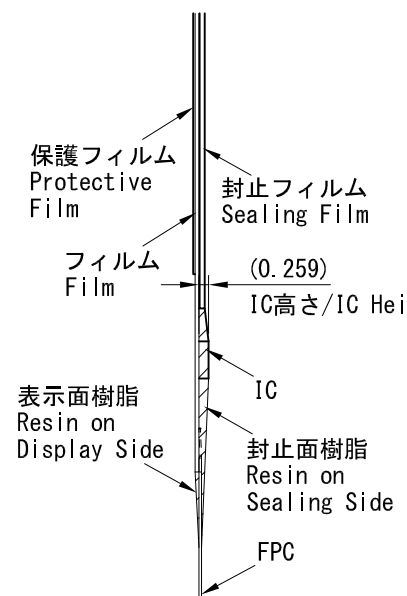
B部拡大図 (5 : 1) B-Portion Magnified Drawing (5:1)
